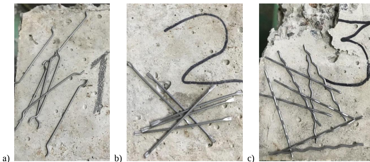
Fig. 1. Types of steel fiber used: a – anchor; b – flattened; c – wave
