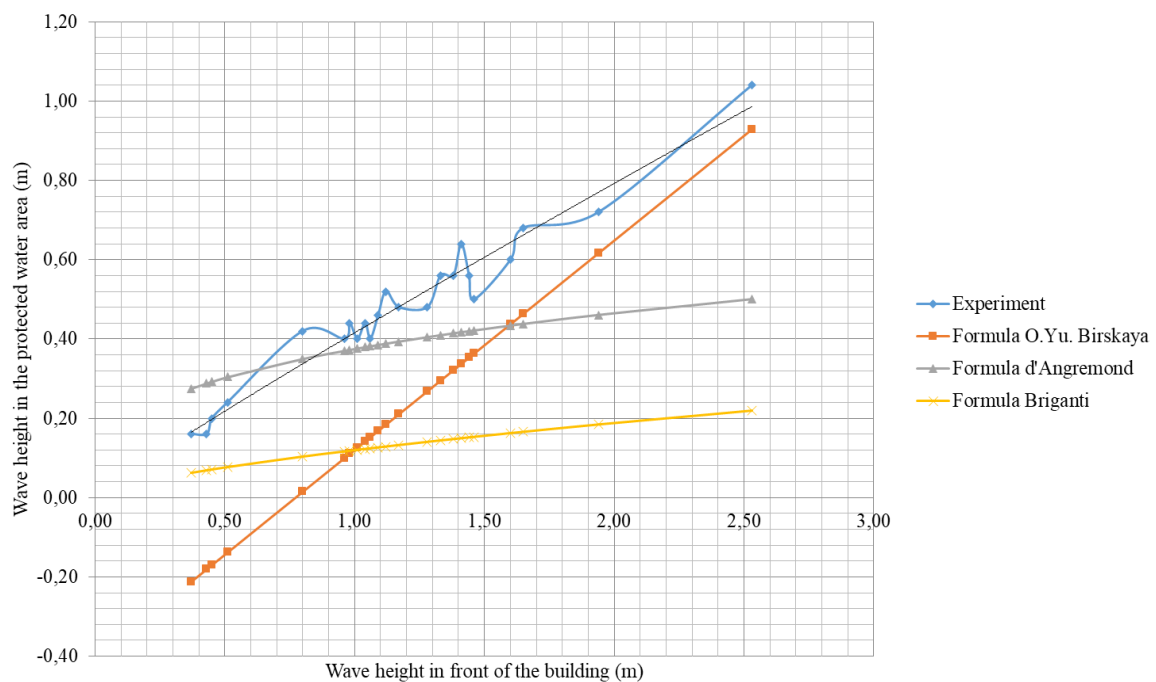
Fig. 5. Parameters of wave transformation at the width of the concrete mass b=6.0 (m) and elevation \Delta H=0 (m)
