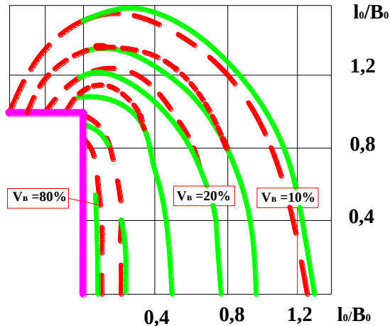
Fig. 3. The distribution of the relative rate of absorption of air in the spectrum of a rectangular pipe speed:
