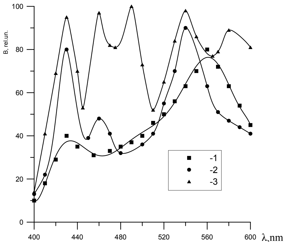
Fig. 2. Spectral distribution of the PL (1), electroluminescence (2) and LEIE (3) Ta_2O_5 films.
