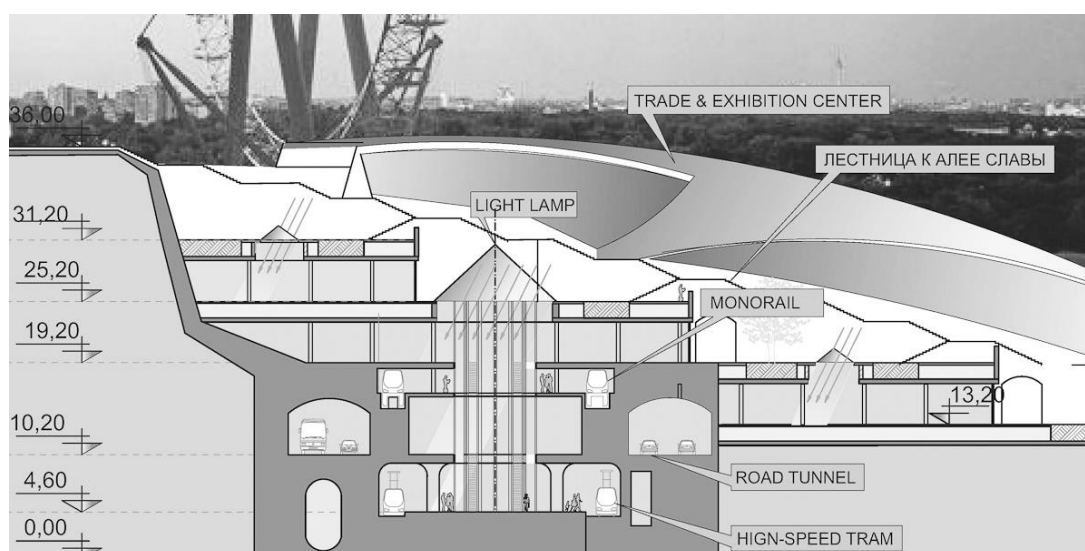
Fig 3. The transfer station of the high-speed tram on a monorail integrated into slopes
