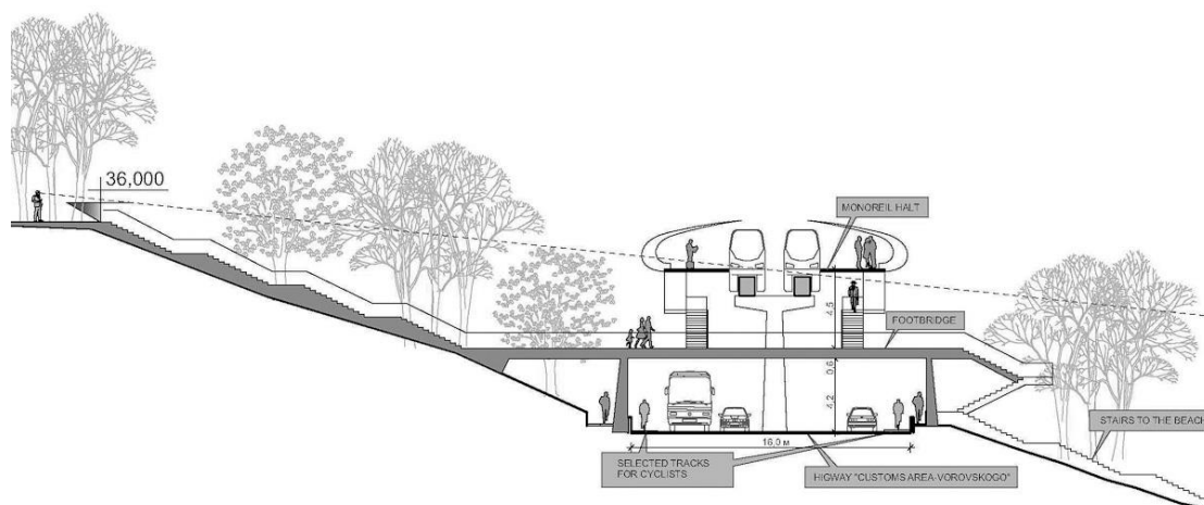
The fig. 2 Scheme of the Organization of the Overpass on slopes
