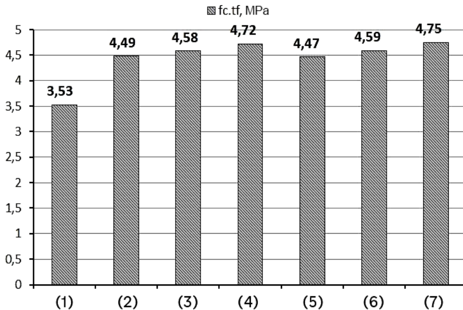
Fig. 3. Tensile strength of bending concrete
