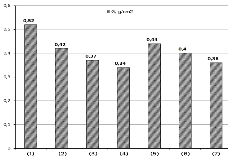
Fig. 6. The abrasion index of the studied samples of concrete and fiber concrete
