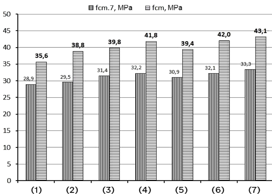
Fig. 1. Compressive strength of concrete at the age of 7 and 28 days
